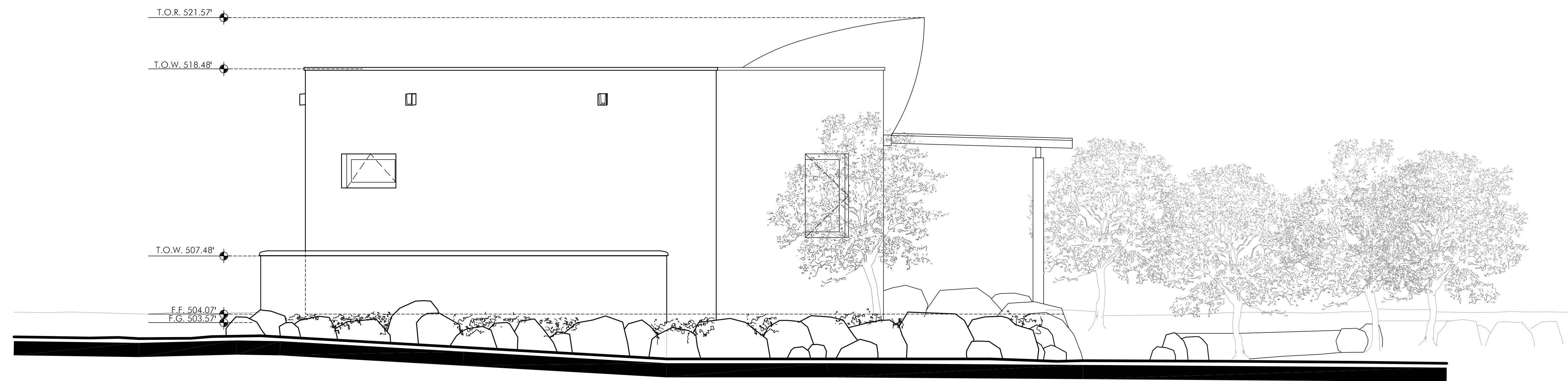
SOUTHWEST ELEVATION
